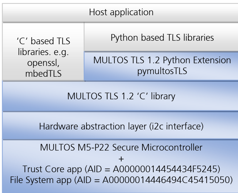
Figure 1 - Software Stack
